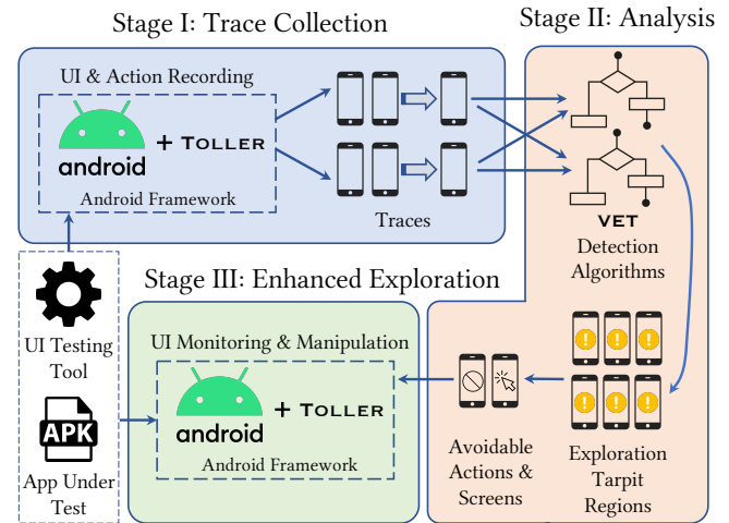
Figure 2: Overview of VET.
